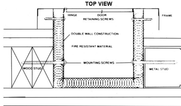
TWO HOUR WALL SYSTEM
