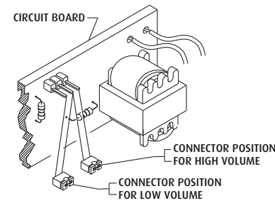
JUMPER LOCATION FOR VOLUME SETTINGS
