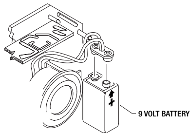
VIEW SHOWING BATTERY REPLACEMENT
